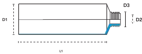
Cylindrical aluminium tubes
